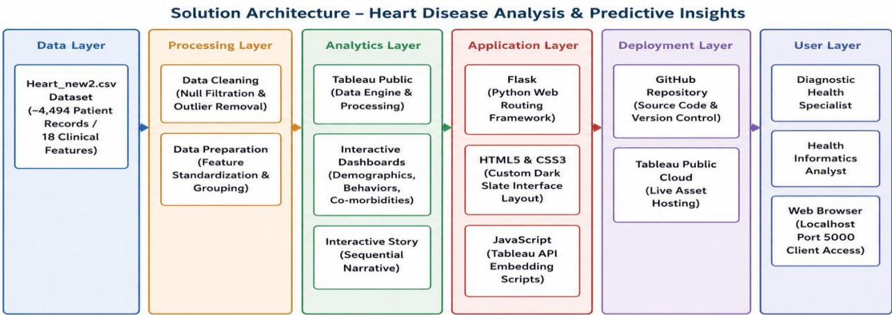
Figure 1: Architecture and data flow of the Heart Disease Analysis & Predictive Insights analytics application
